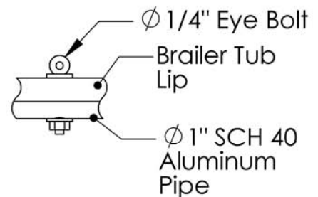
Brace Detail
